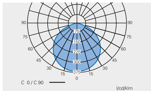
Polar curve LPL LED-C60-150W, 6000 K
