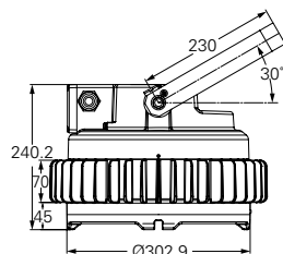
Mounting bracket
